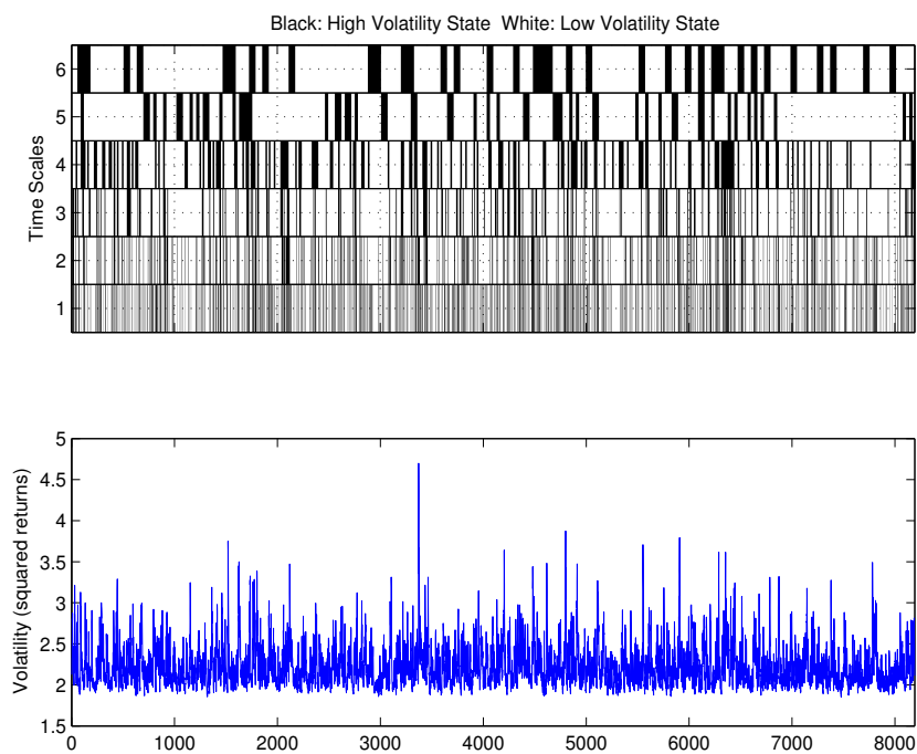
Figure 15: Most likely sequence of states from the fitted wavelet hidden Markov tree (HMT) model for the volatility of the simulated GARCH(1,1) process. The first state S = 0 (light rectangles) indicates a low volatility (state) regime while the second state S = 1 (dark rectangles) indicates a high volatility regime.
