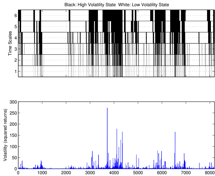
Figure 14: Most likely sequence of states from the fitted wavelet hidden Markov tree (HMT) model for the simulated fractionally differenced stochastic volatility process. The first state S = 0 (light rectangles) indicates a low volatility (state) regime while the second state S = 1 (dark rectangles) indicates a high volatility regime.
