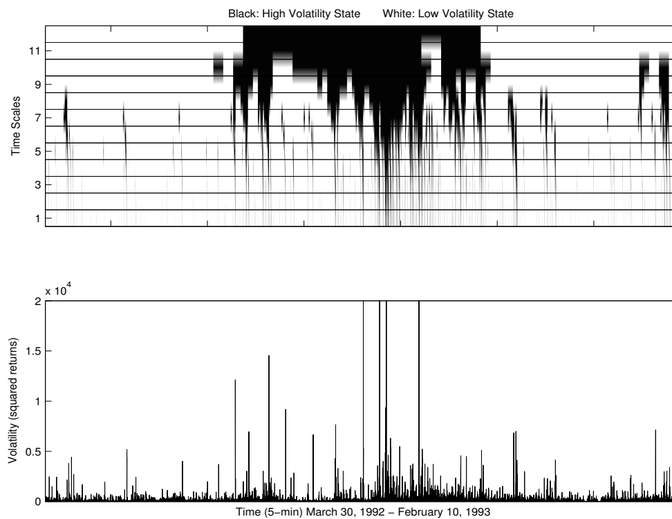
Figure 12: Most likely sequence of states from the fitted wavelet hidden Markov tree (HMT) model from March 1992 to February 1993 for the USD-DEM volatility. The first state S = 0 (light rectangles) indicates a low volatility (state) regime while the second state S = 1 (dark rectangles) indicates a high volatility regime.
